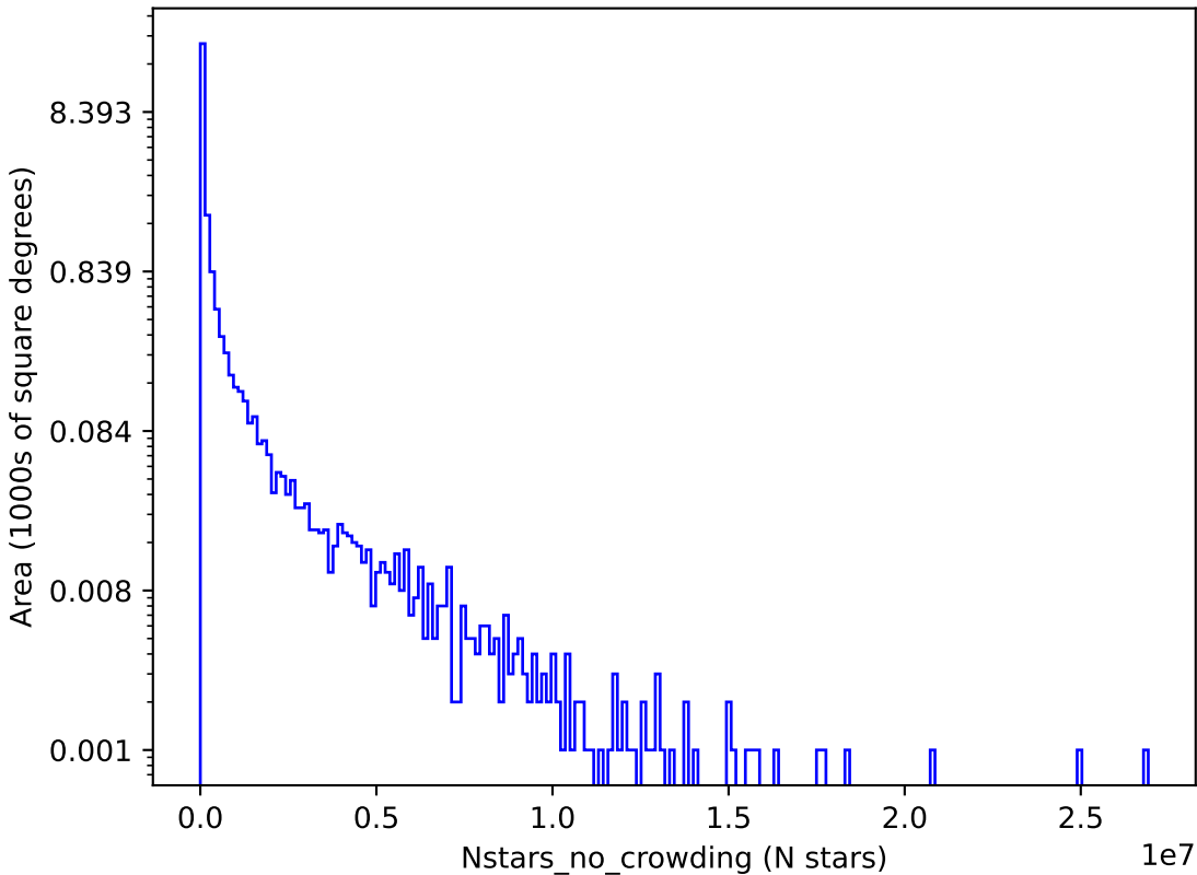
too_combined_s2.0_v3.4_10yrs z: Nstars_no_crowding
