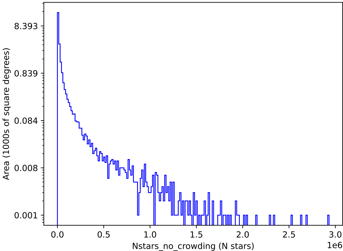
too_combined_s2.0_v3.4_10yrs u: Nstars_no_crowding
