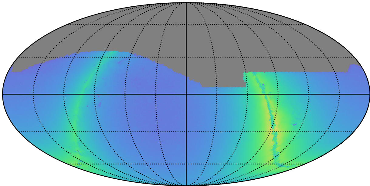
too_combined_s2.0_v3.4_10yrs r: Nstars_no_crowding
