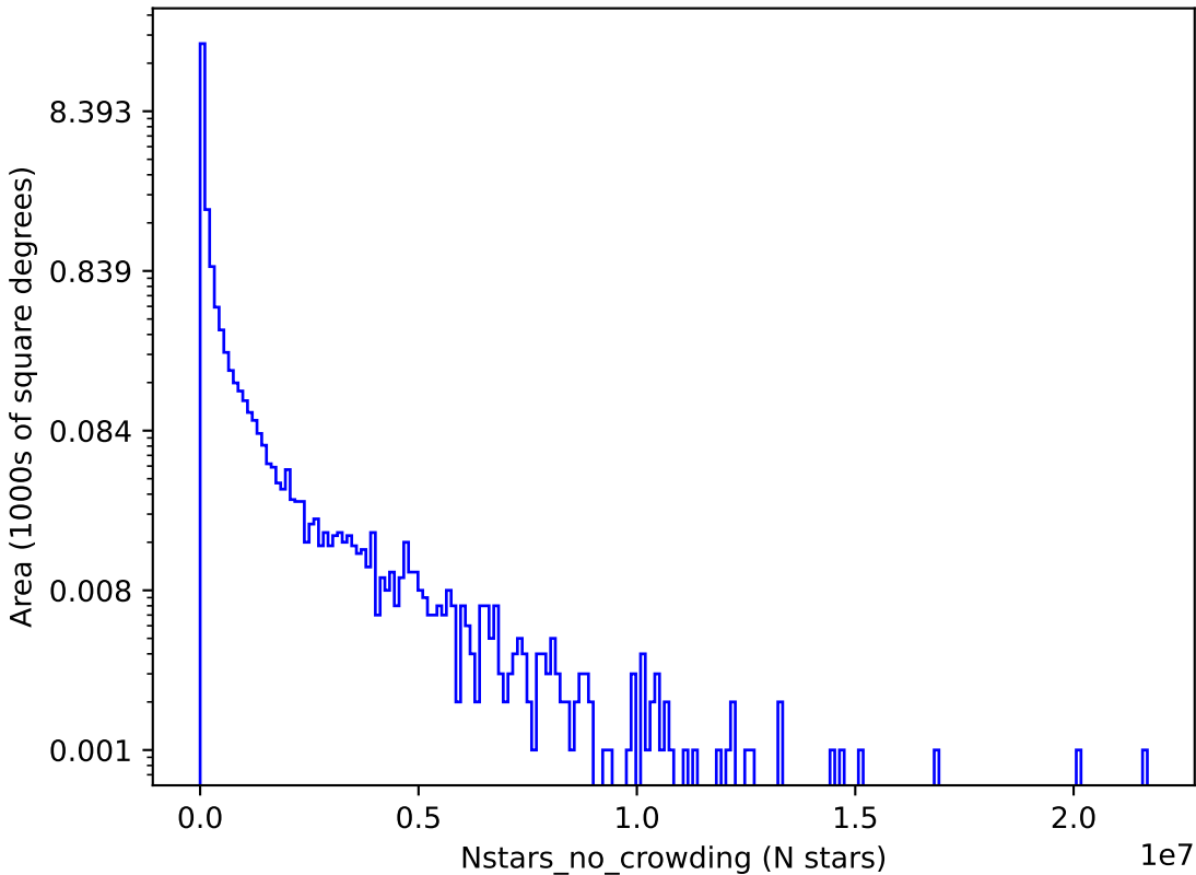
too_combined_s2.0_v3.4_10yrs r: Nstars_no_crowding
