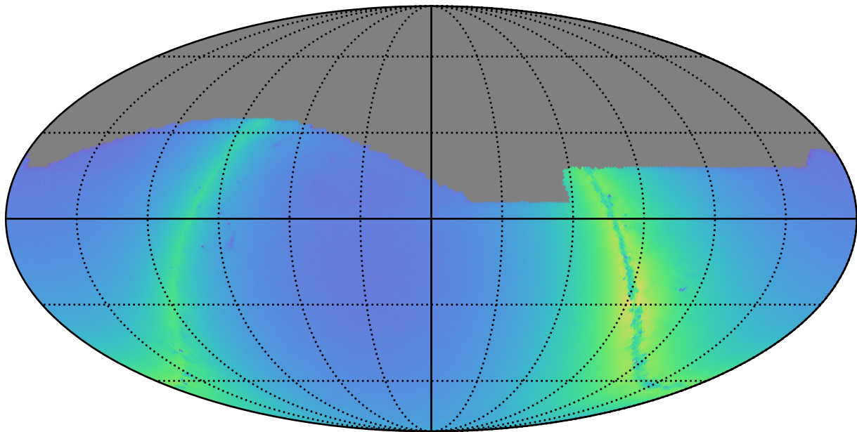
too_combined_s2.0_v3.4_10yrs i: Nstars_no_crowding
