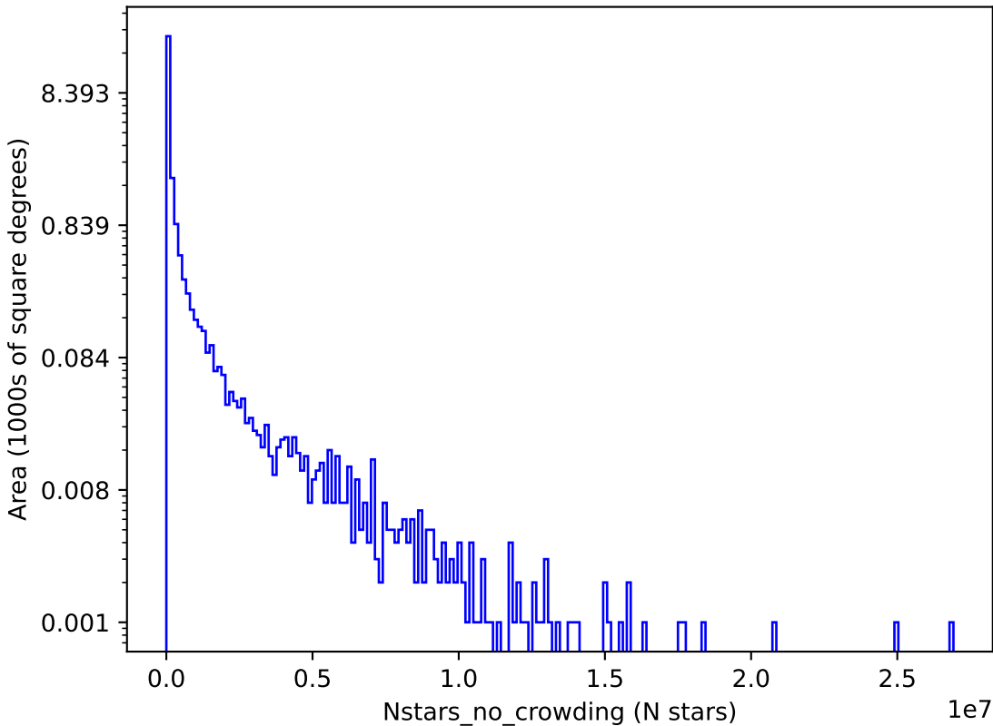
too_combined_s2.0_v3.4_10yrs i: Nstars_no_crowding
