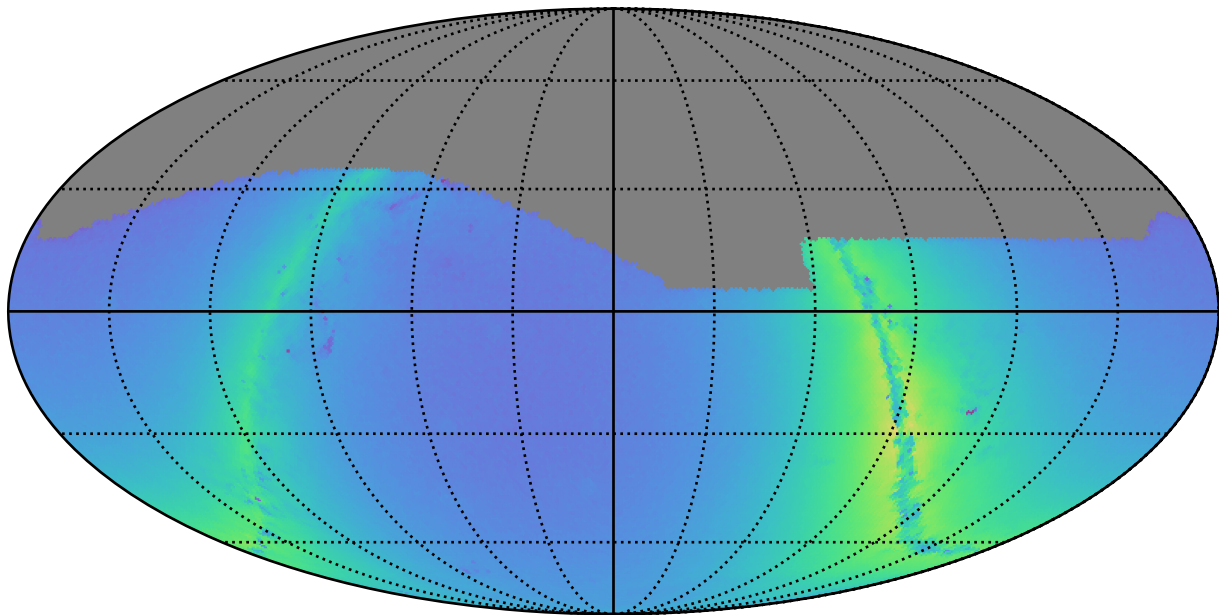
too_combined_s2.0_v3.4_10yrs g: Nstars_no_crowding
