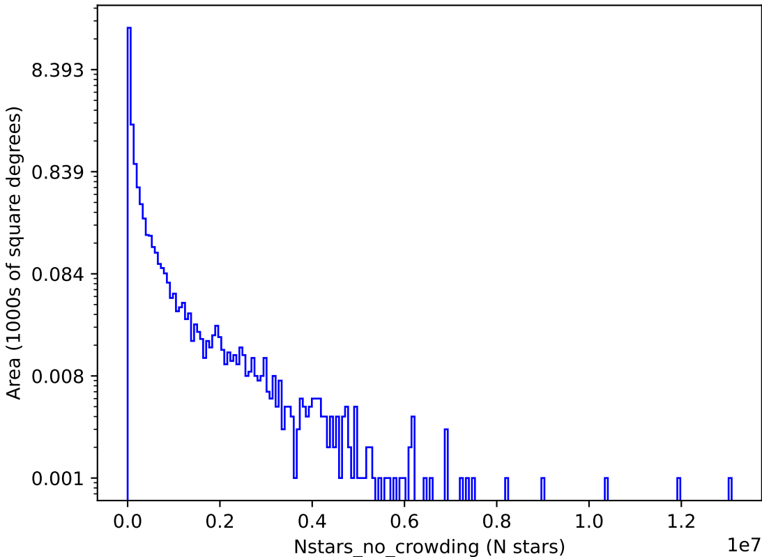
too_combined_s2.0_v3.4_10yrs g: Nstars_no_crowding
