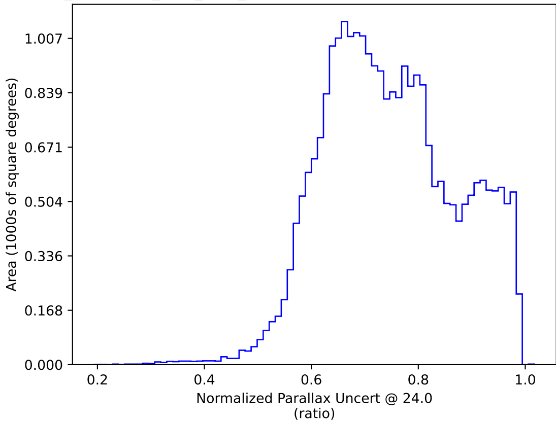
too_combined_s2.0_v3.4_10yrs : Normalized Parallax Uncert @ 24.0
