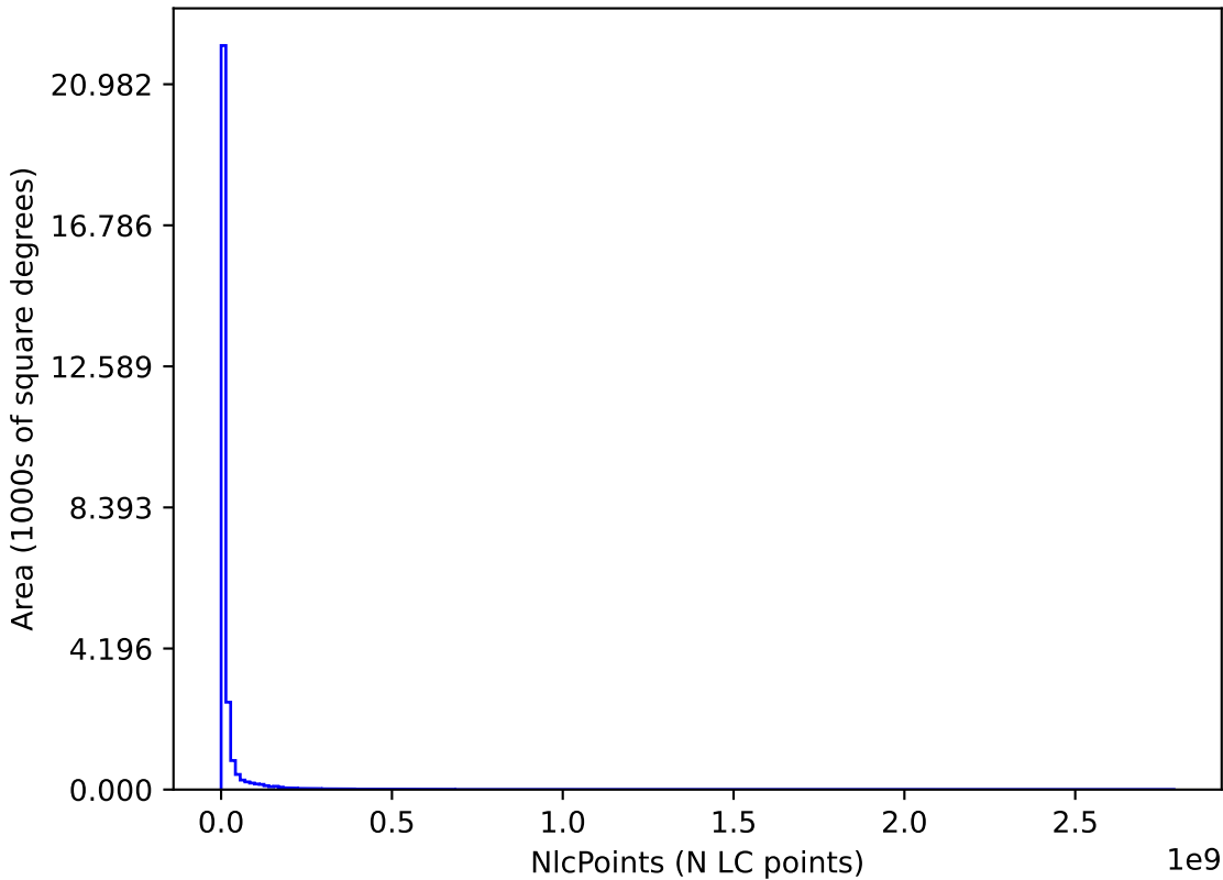
too_combined_s2.0_v3.4_10yrs : NlcPoints
