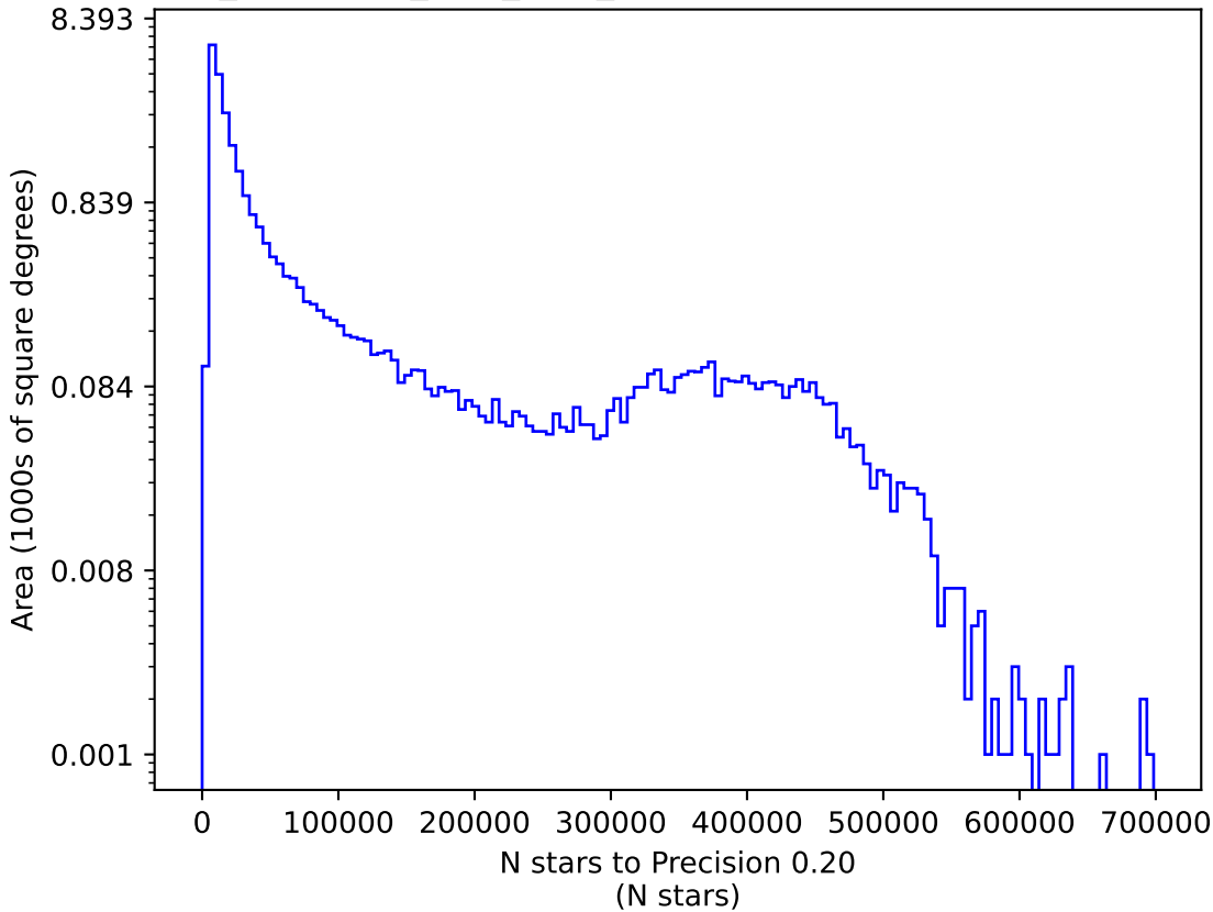
too_combined_s2.0_v3.4_10yrs z: N stars to Precision 0.20
