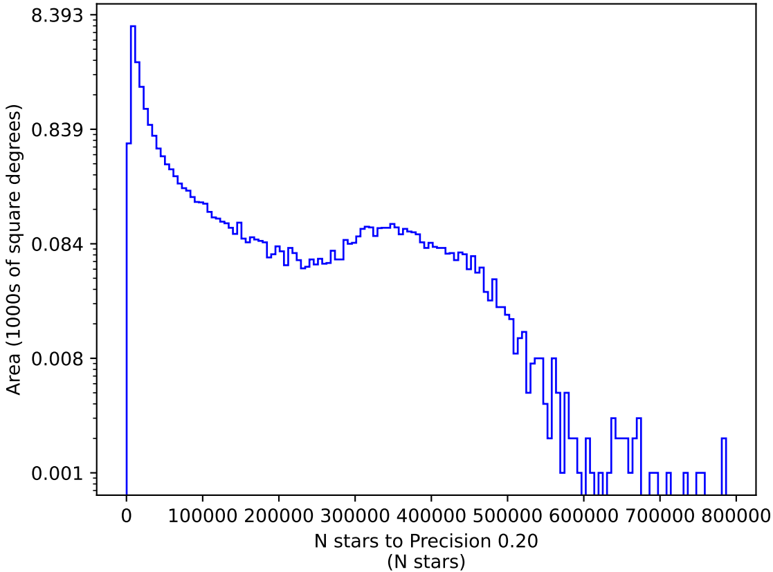
too_combined_s2.0_v3.4_10yrs y: N stars to Precision 0.20
