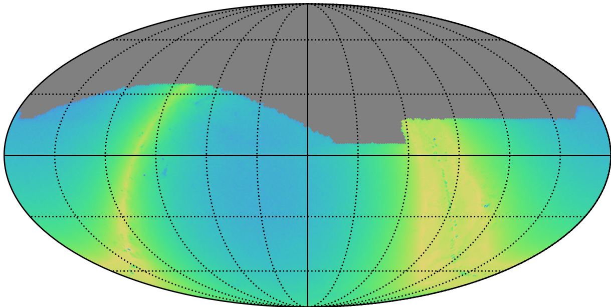
too_combined_s2.0_v3.4_10yrs i: N stars to Precision 0.20
