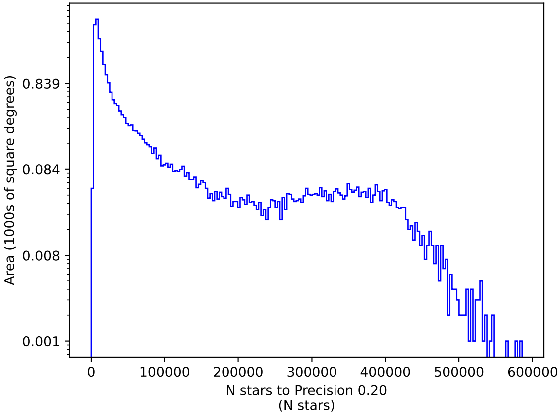
too_combined_s2.0_v3.4_10yrs g: N stars to Precision 0.20
