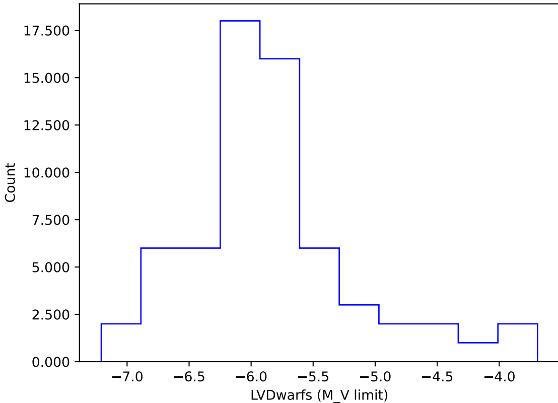
too_combined_s2.0_v3.4_10yrs gi: LVDwarfs
