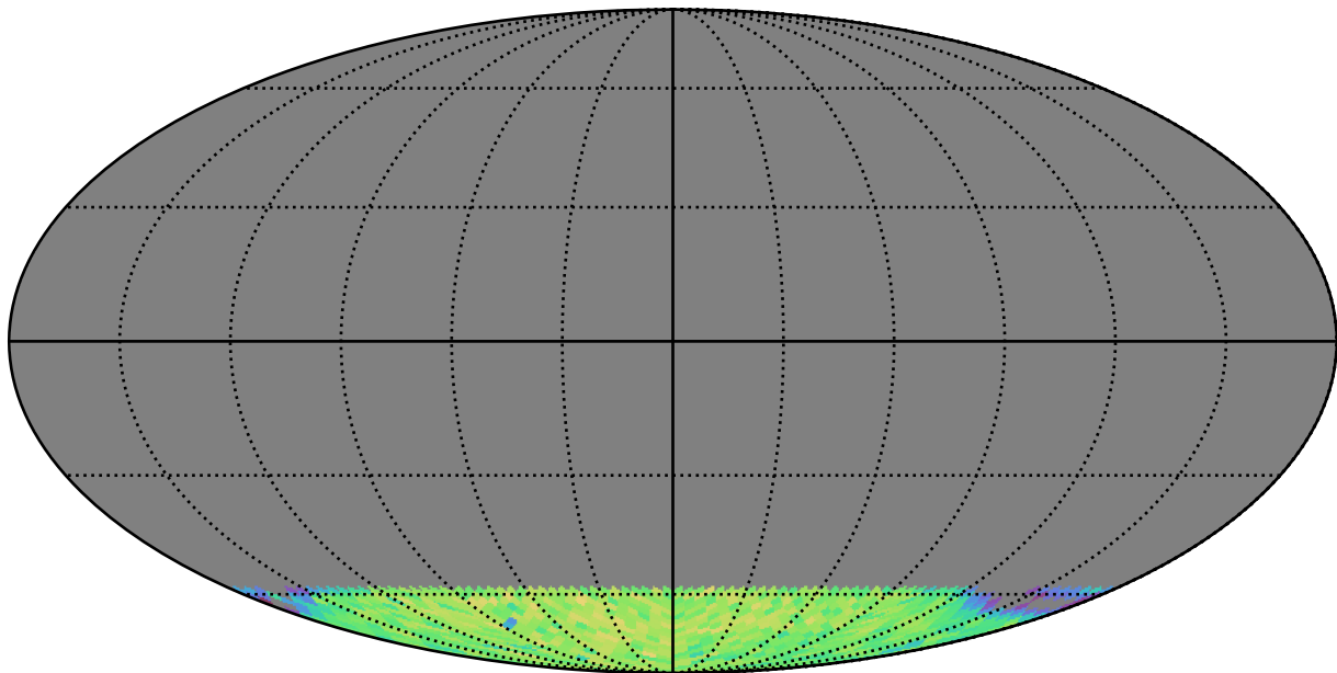
too_combined_s2.0_v3.4_10yrs gi SCP: LVDwarfs
