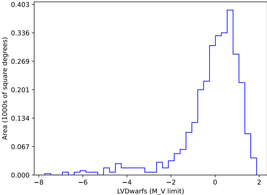
too_combined_s2.0_v3.4_10yrs gi SCP: LVDwarfs
