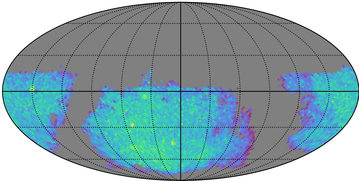
too_combined_s2.0_v3.4_10yrs gi: LVDwarfs
