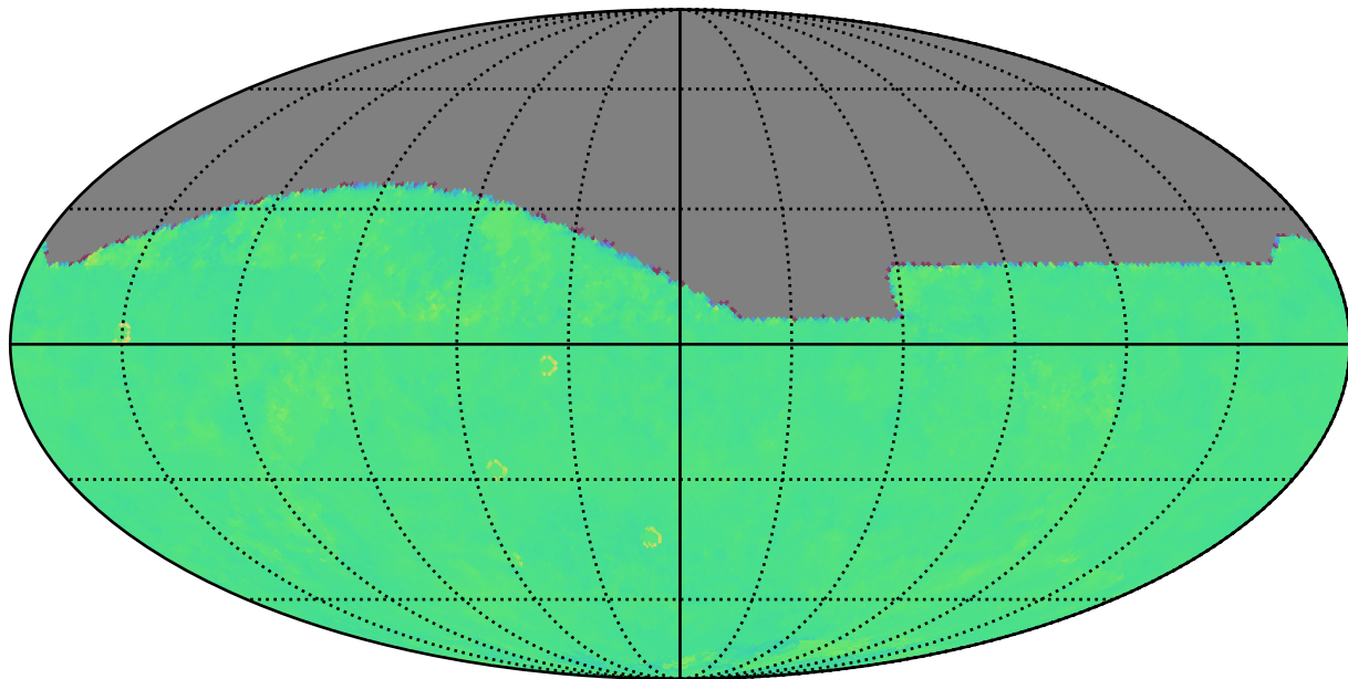
too_combined_s2.0_v3.4_10yrs z: Kuiper rotTelPos
