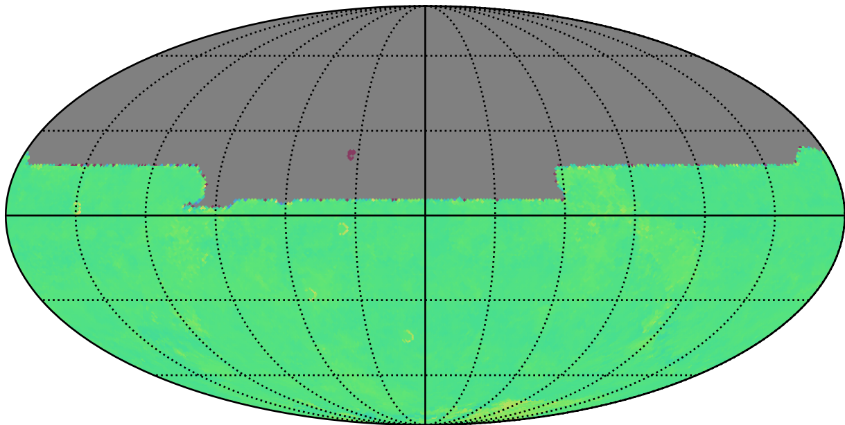
too_combined_s2.0_v3.4_10yrs y: Kuiper rotTelPos
