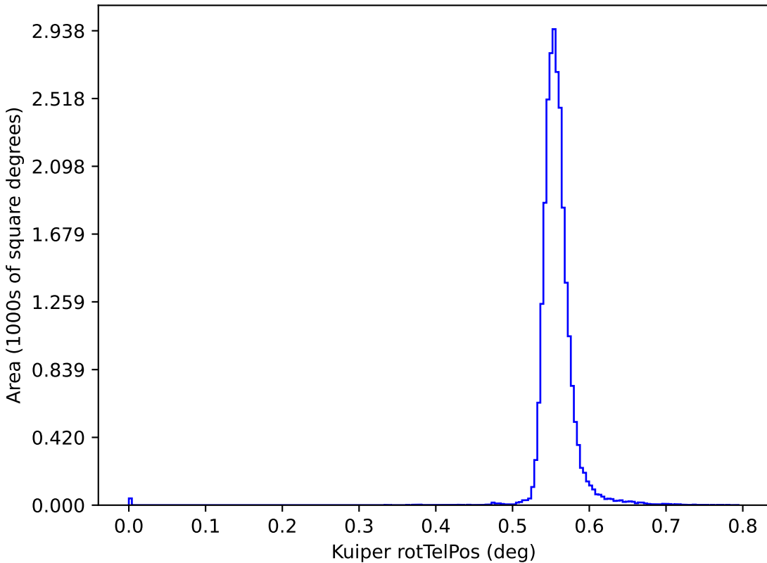
too_combined_s2.0_v3.4_10yrs y: Kuiper rotTelPos
