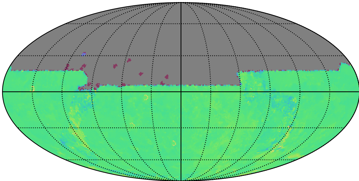
too_combined_s2.0_v3.4_10yrs u: Kuiper rotTelPos
