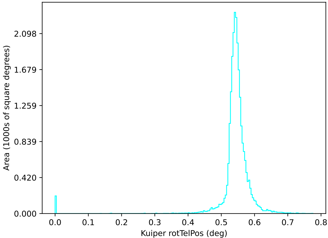
too_combined_s2.0_v3.4_10yrs u: Kuiper rotTelPos
