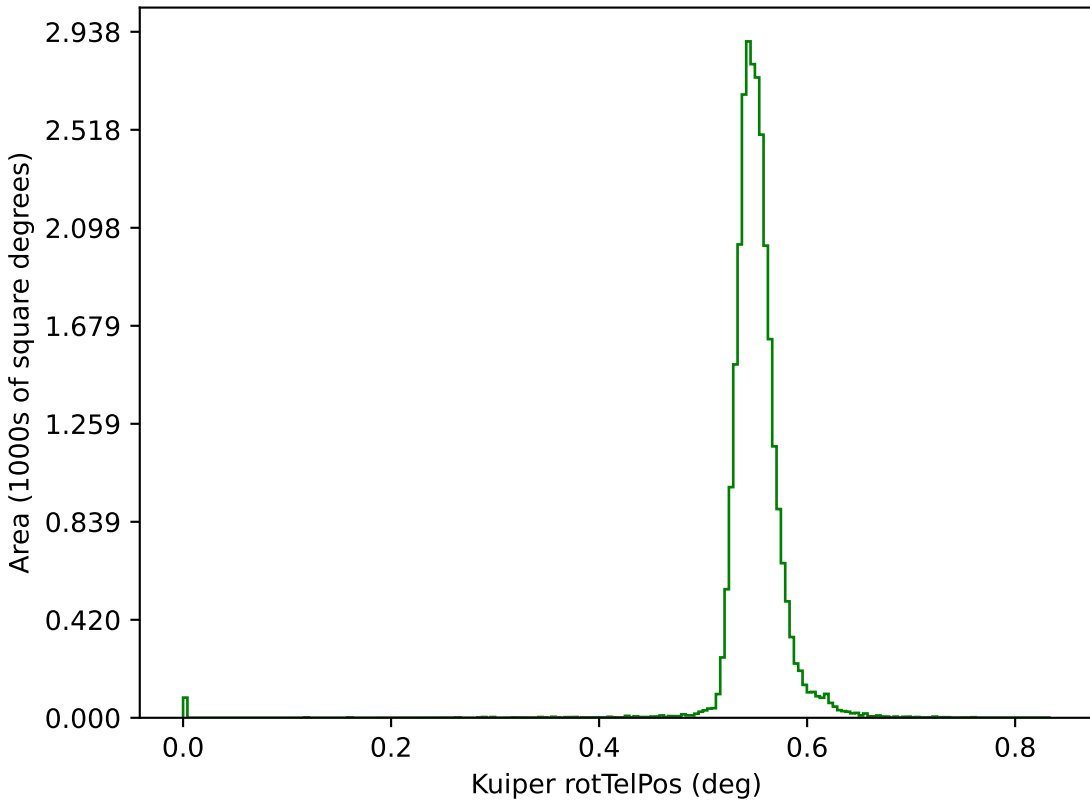
too_combined_s2.0_v3.4_10yrs g: Kuiper rotTelPos
