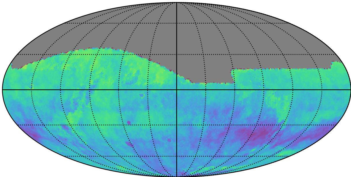
too_combined_s2.0_v3.4_10yrs z: Kuiper rotSkyPos
