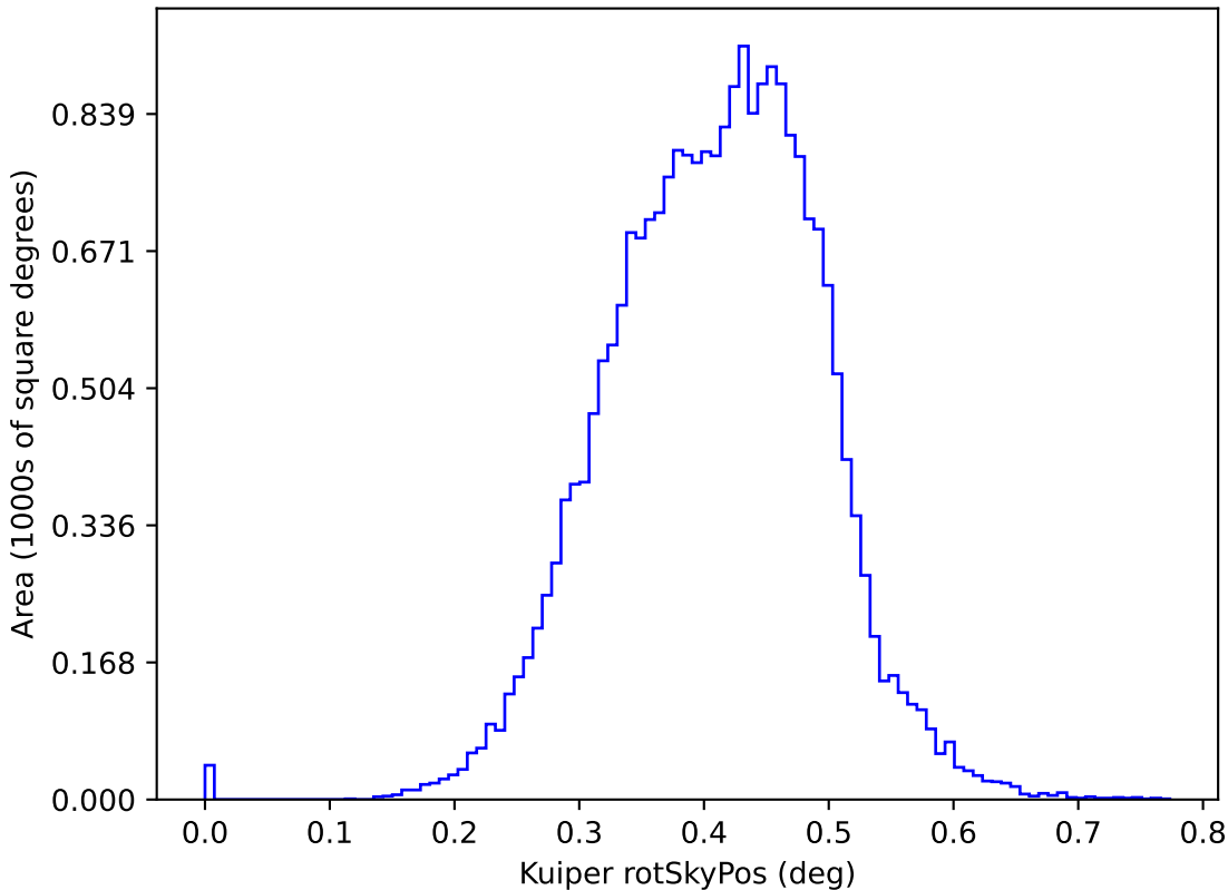
too_combined_s2.0_v3.4_10yrs y: Kuiper rotSkyPos
