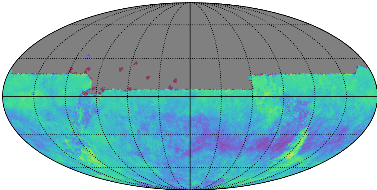
too_combined_s2.0_v3.4_10yrs u: Kuiper rotSkyPos
