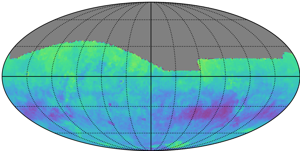
too_combined_s2.0_v3.4_10yrs r: Kuiper rotSkyPos
