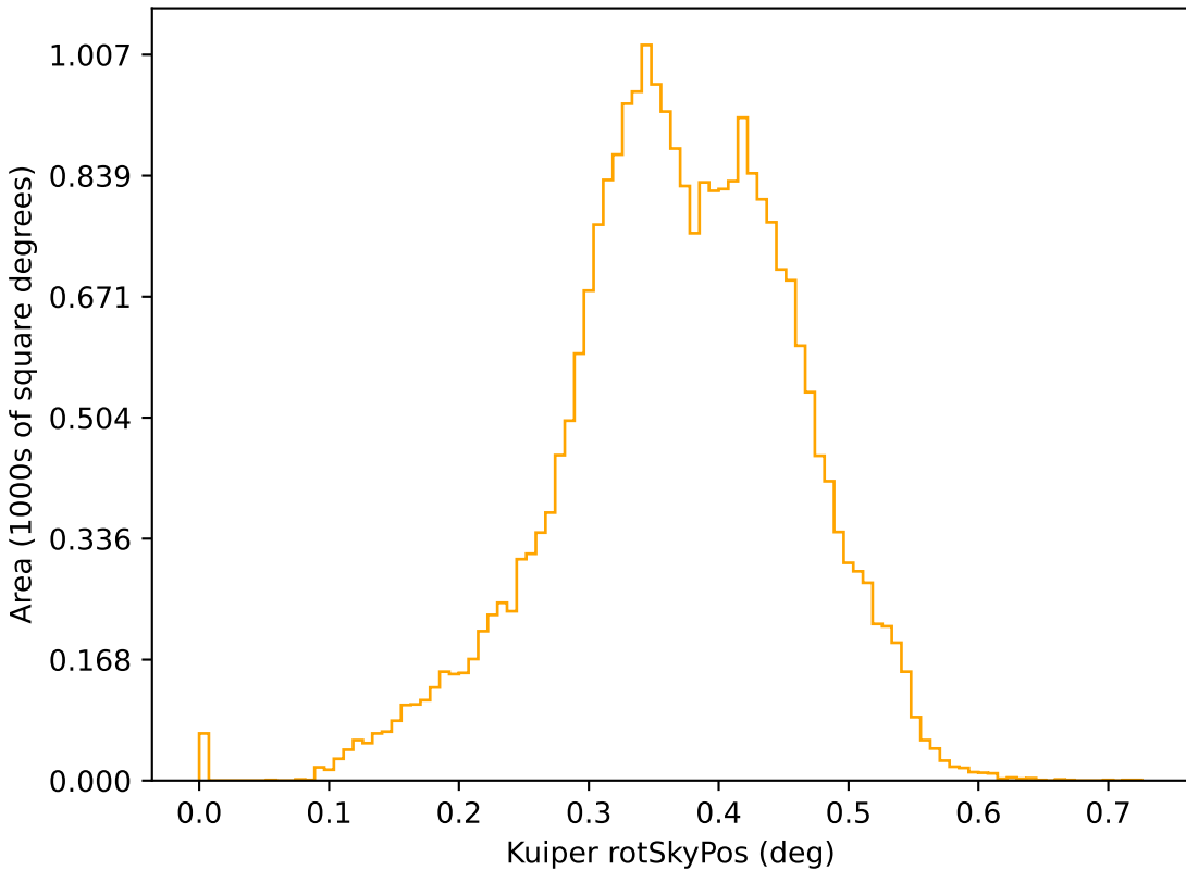
too_combined_s2.0_v3.4_10yrs r: Kuiper rotSkyPos
