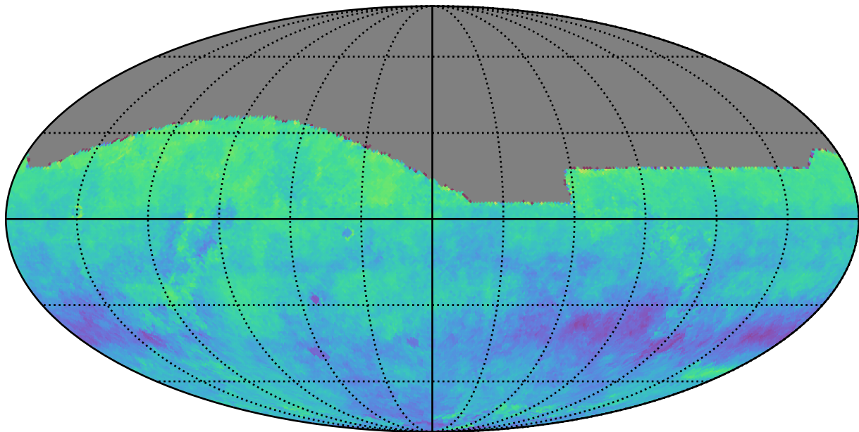
too_combined_s2.0_v3.4_10yrs i: Kuiper rotSkyPos
