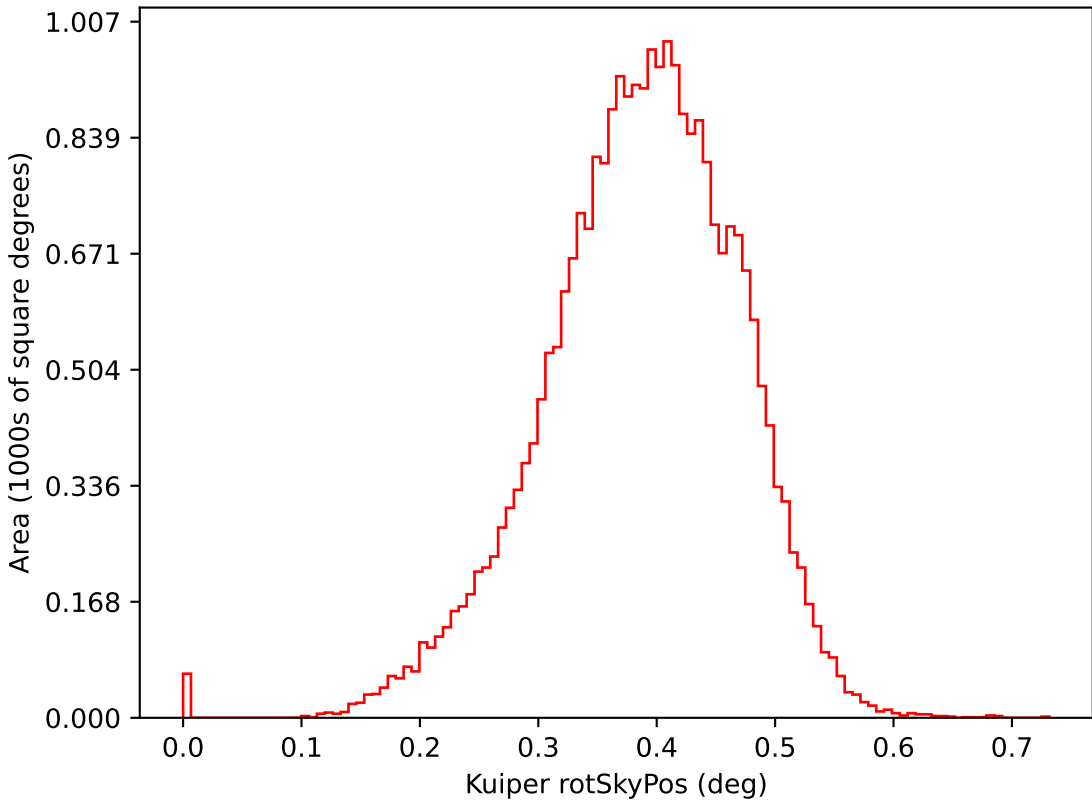
too_combined_s2.0_v3.4_10yrs i: Kuiper rotSkyPos
