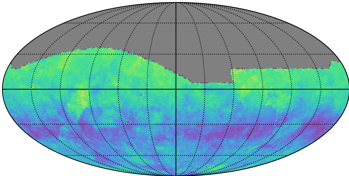
too_combined_s2.0_v3.4_10yrs g: Kuiper rotSkyPos
