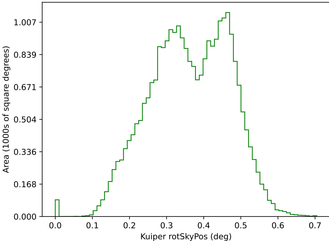
too_combined_s2.0_v3.4_10yrs g: Kuiper rotSkyPos
