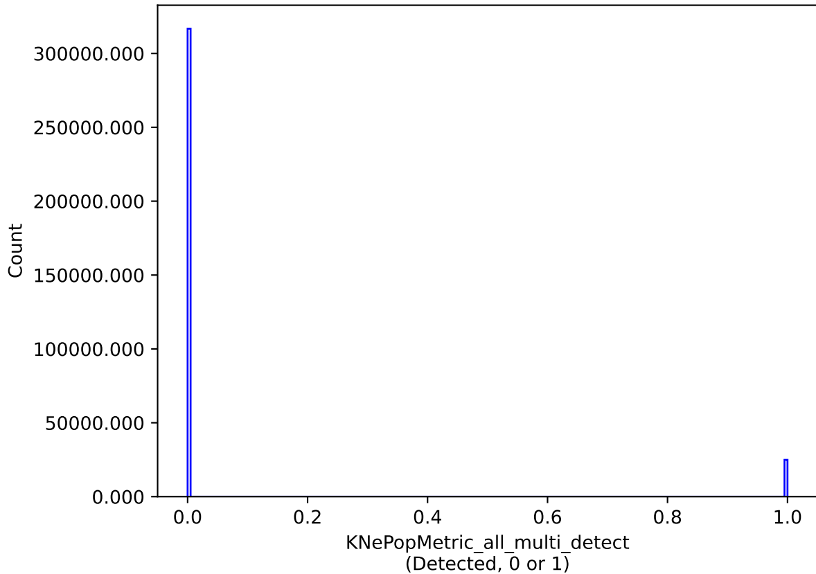
too_combined_s2.0_v3.4_10yrs all models: KNePopMetric_all_multi_detect
