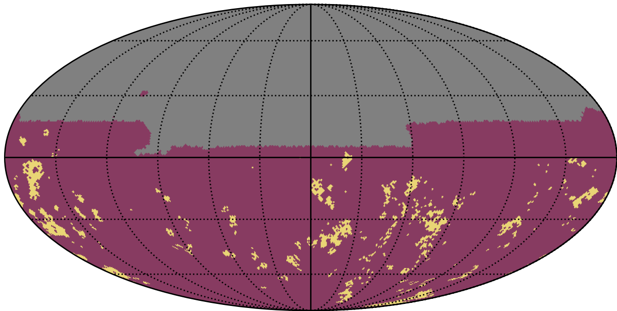
too_combined_s2.0_v3.4_10yrs u band: Gaps_7hr
