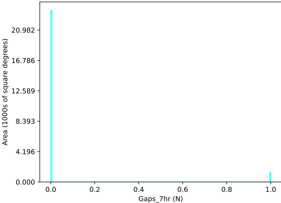
too_combined_s2.0_v3.4_10yrs u band: Gaps_7hr
