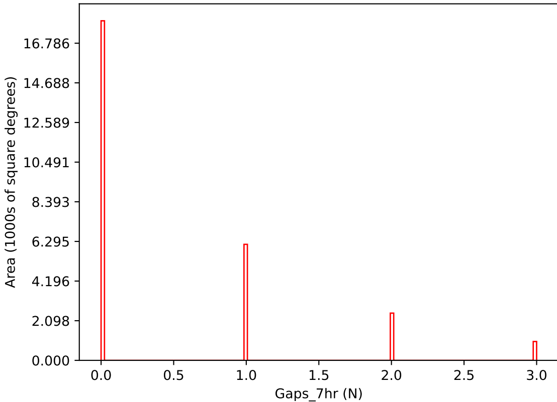
too_combined_s2.0_v3.4_10yrs i band: Gaps_7hr
