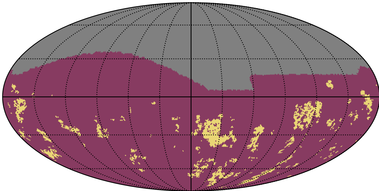
too_combined_s2.0_v3.4_10yrs g band: Gaps_7hr
