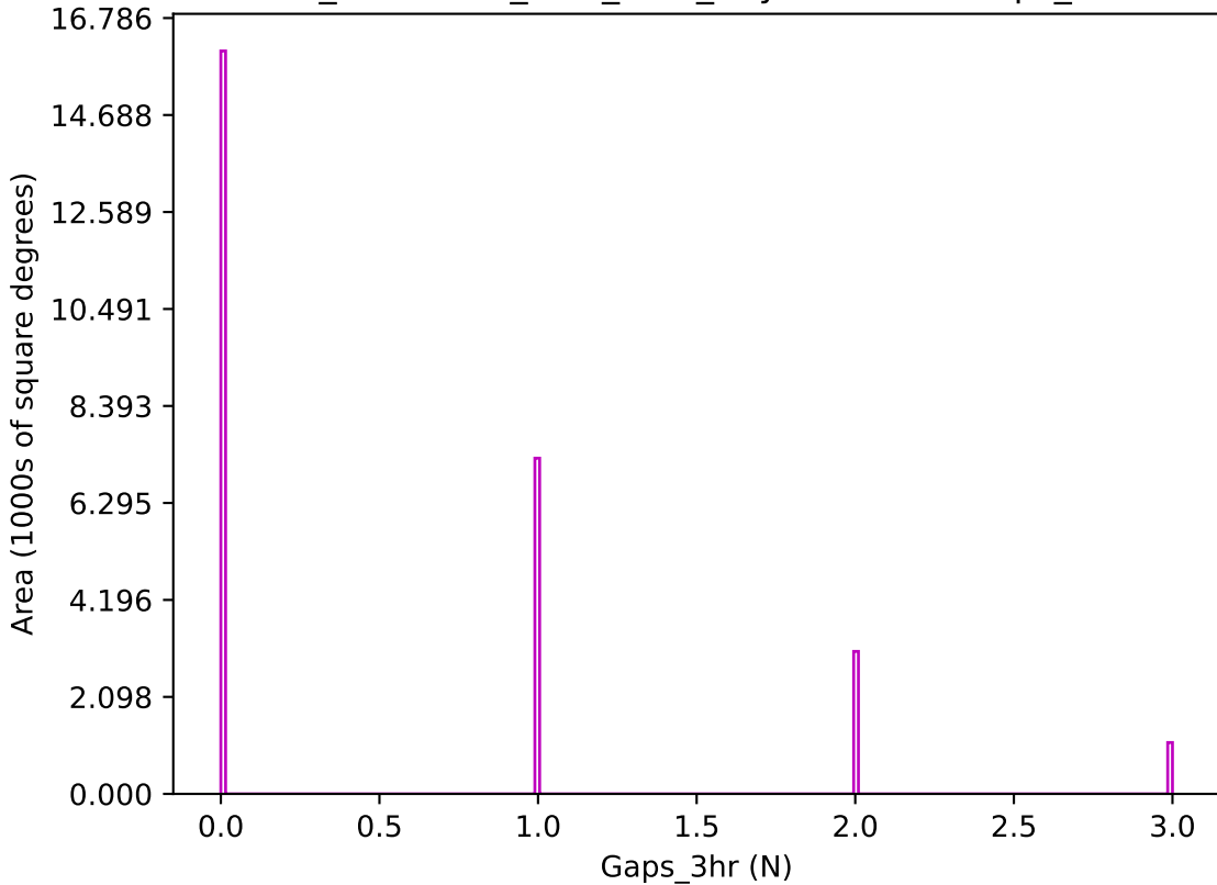
too_combined_s2.0_v3.4_10yrs z band: Gaps_3hr
