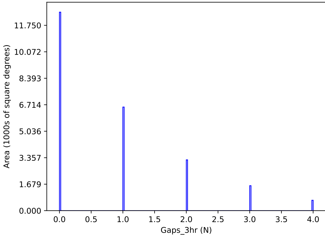
too_combined_s2.0_v3.4_10yrs y band: Gaps_3hr
