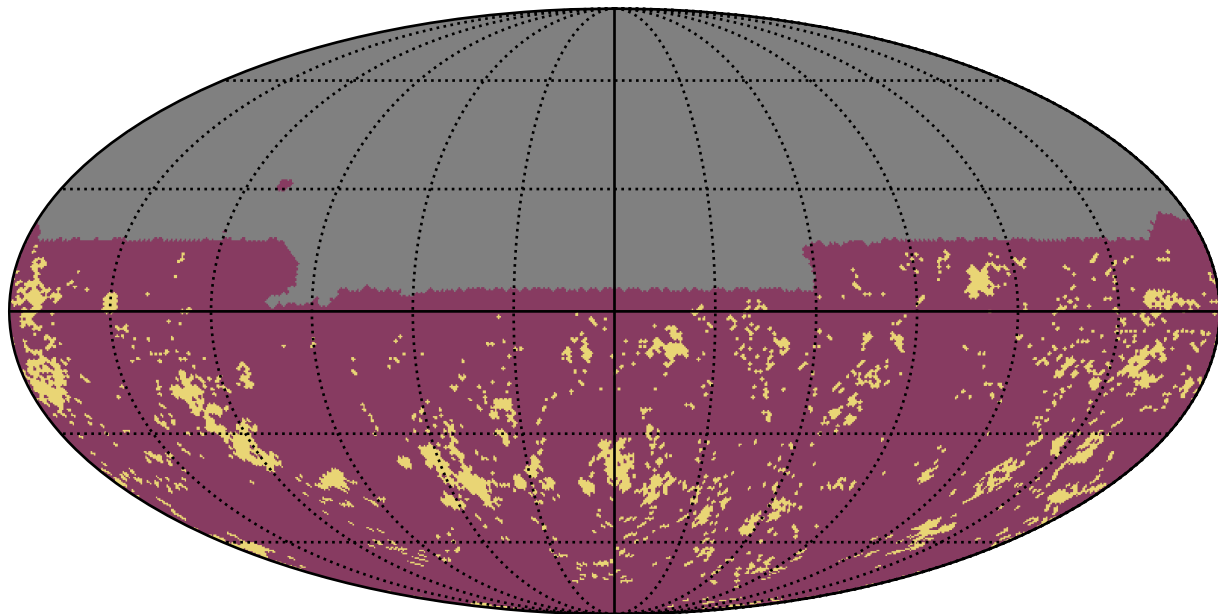
too_combined_s2.0_v3.4_10yrs u band: Gaps_3hr
