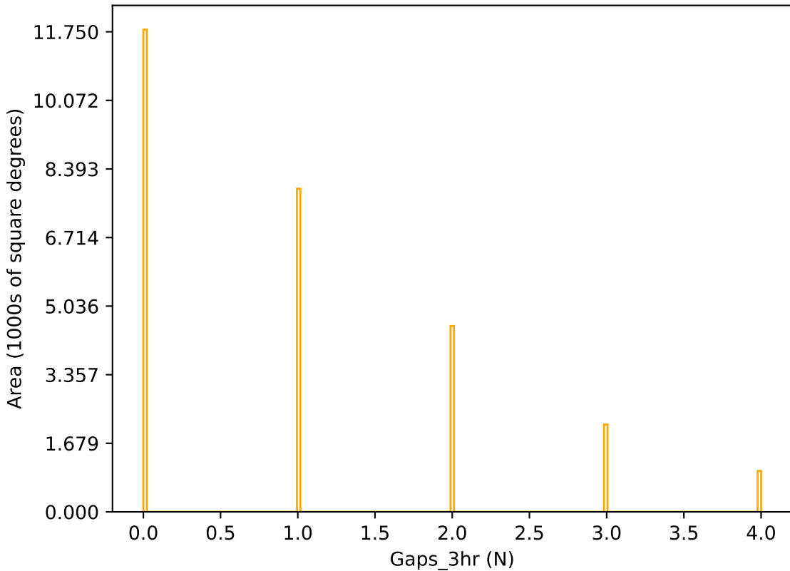
too_combined_s2.0_v3.4_10yrs r band: Gaps_3hr
