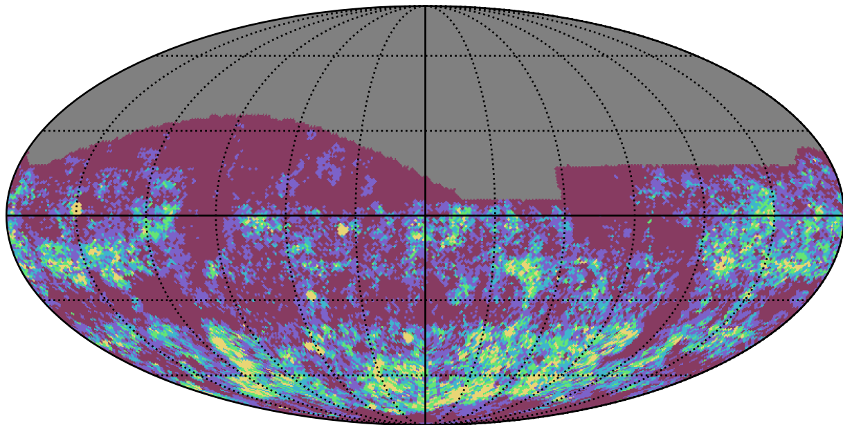
too_combined_s2.0_v3.4_10yrs i band: Gaps_3hr
