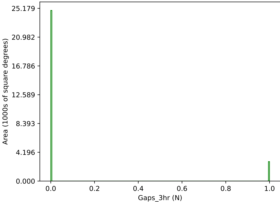
too_combined_s2.0_v3.4_10yrs g band: Gaps_3hr
