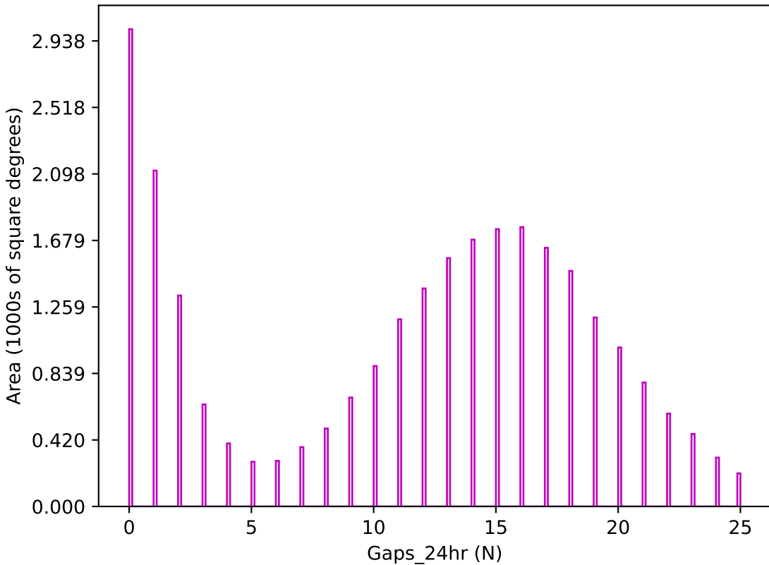
too_combined_s2.0_v3.4_10yrs z band: Gaps_24hr
