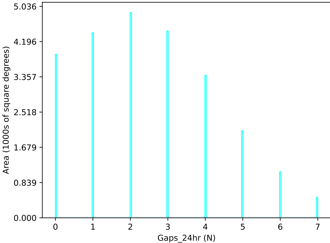
too_combined_s2.0_v3.4_10yrs u band: Gaps_24hr
