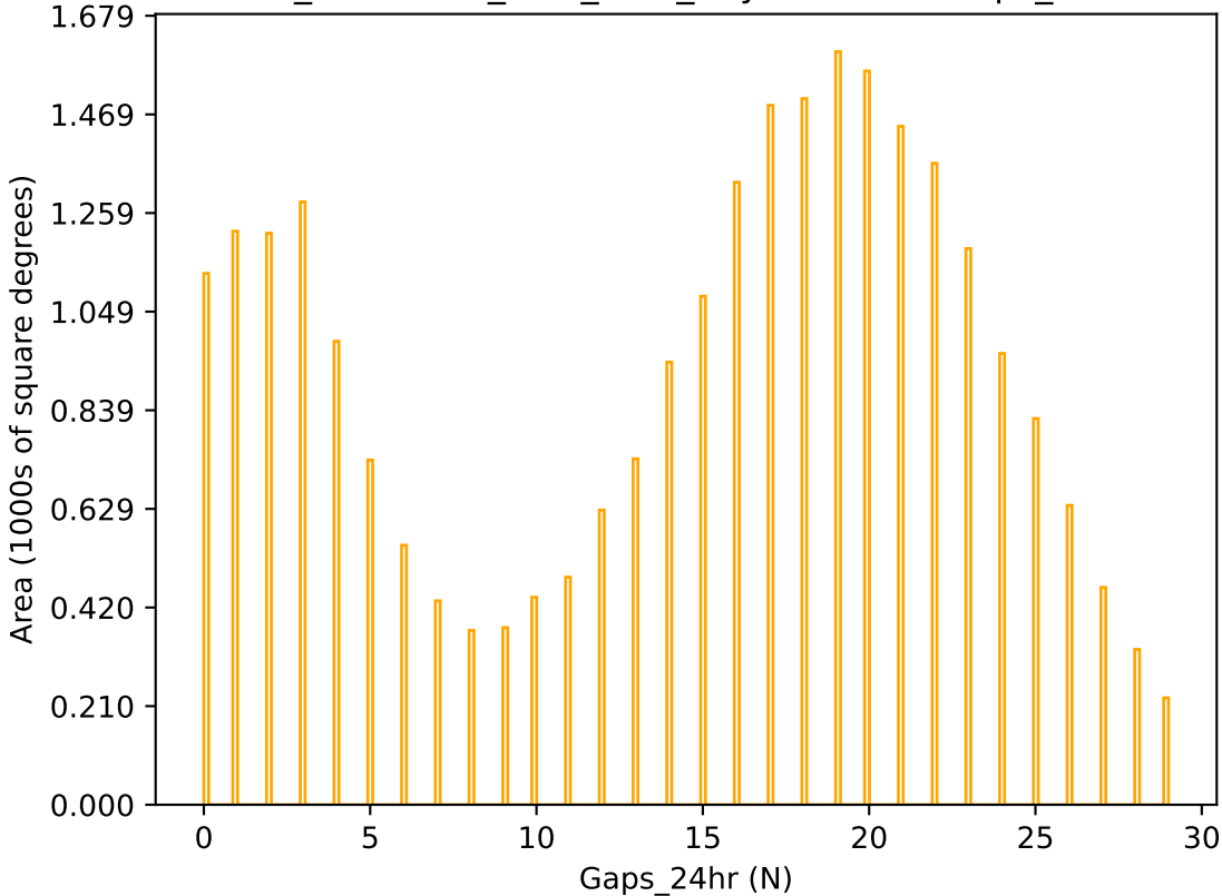
too_combined_s2.0_v3.4_10yrs r band: Gaps_24hr
