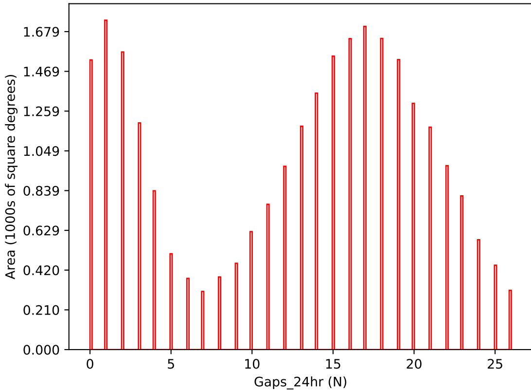
too_combined_s2.0_v3.4_10yrs i band: Gaps_24hr
