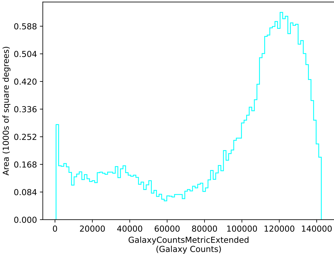
too_combined_s2.0_v3.4_10yrs u: GalaxyCountsMetricExtended
