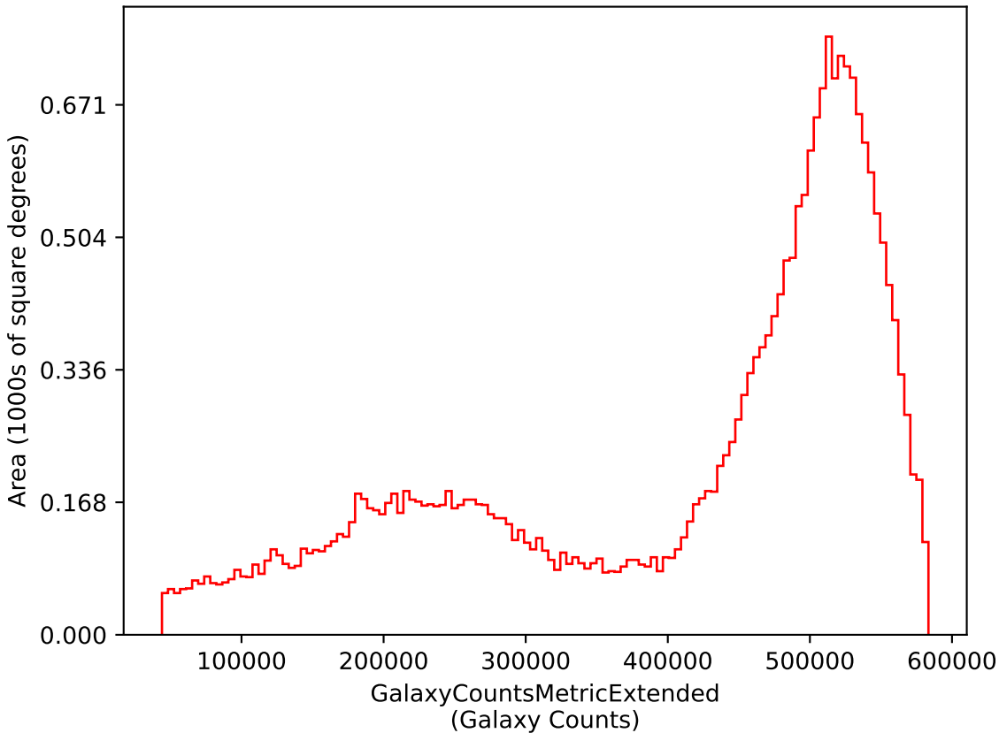
too_combined_s2.0_v3.4_10yrs i: GalaxyCountsMetricExtended
